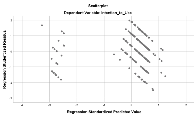
Figure 1. Heteroscedasticity Result
