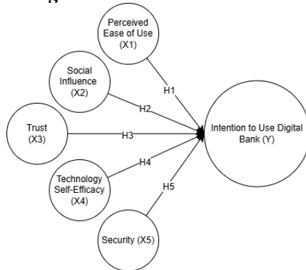
Figure 1. Research Framework
